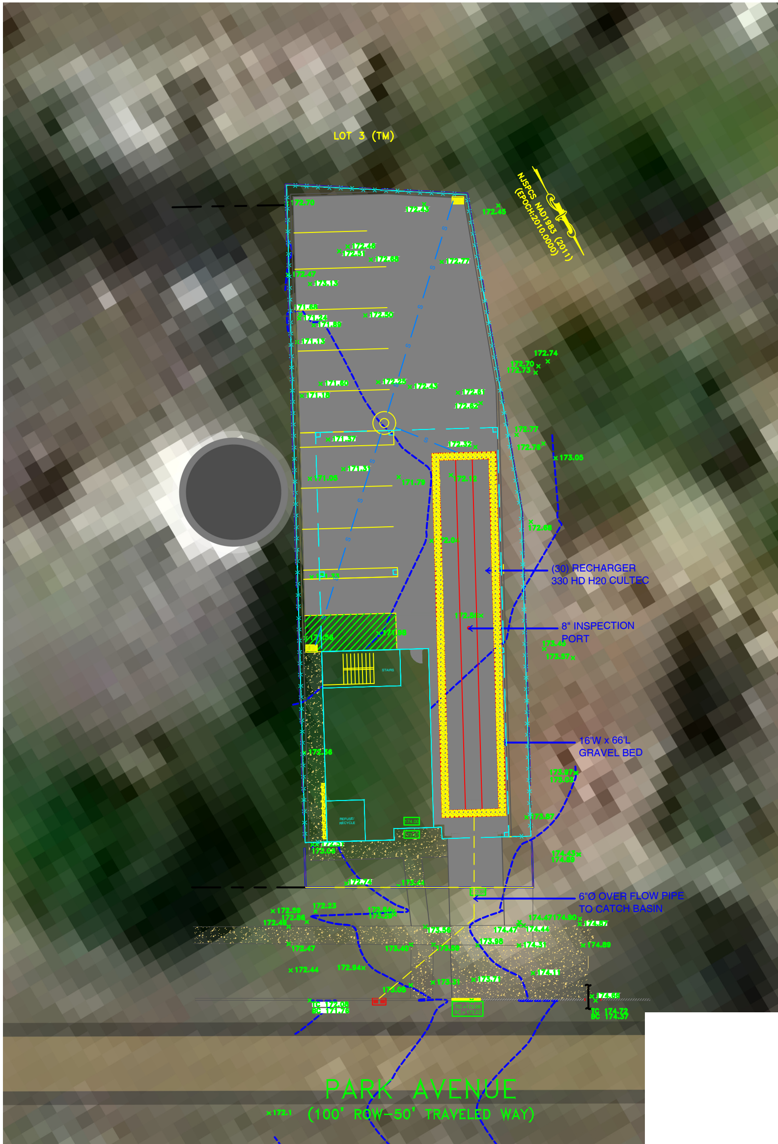
PROPOSED DRAINAGE / GRADING PLAN SCALE: 1" = 15'-0"
