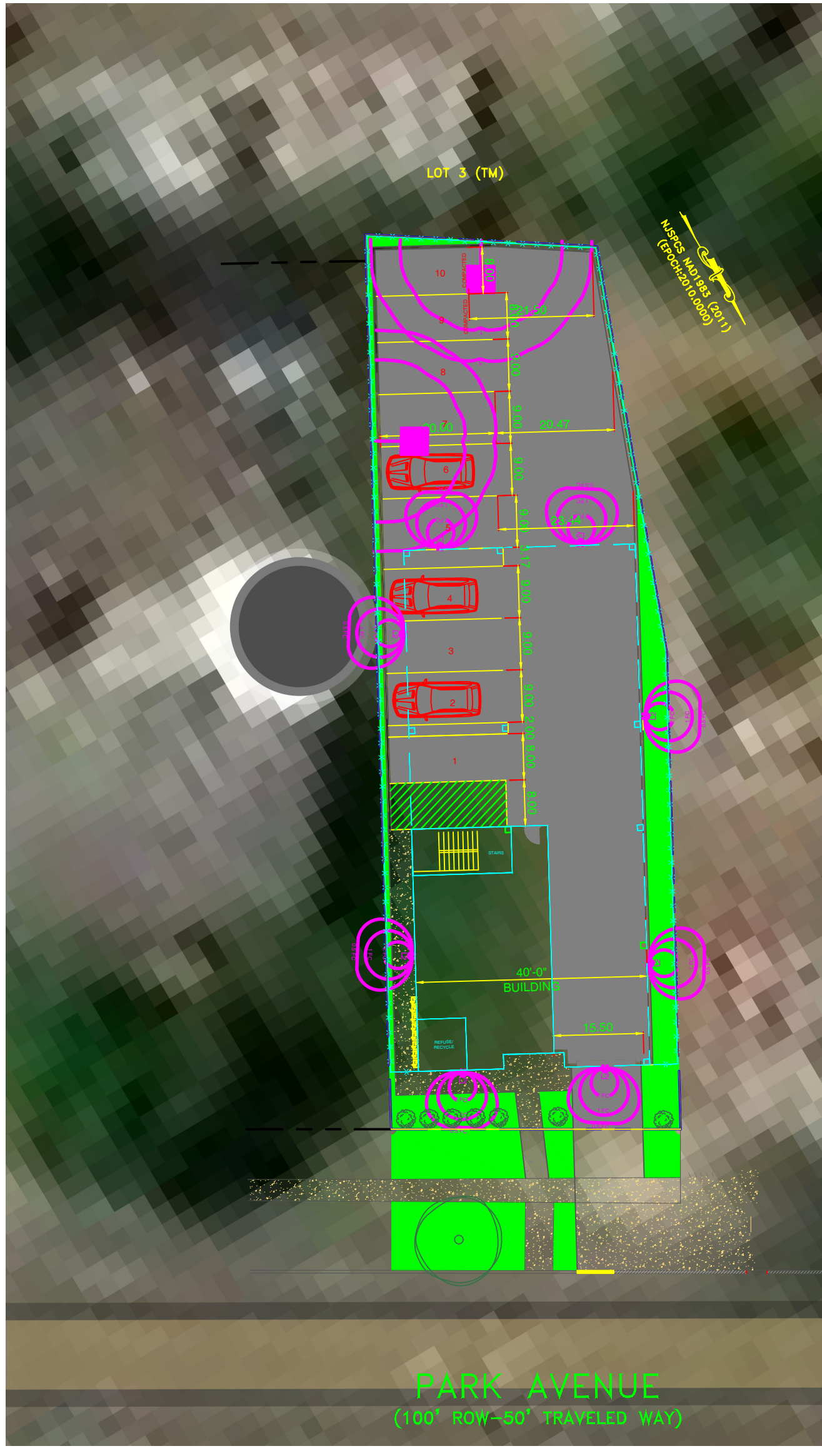
PROPOSED LIGHTING / LANDSCAPING PLAN SCALE: 1" = 15'-0"
