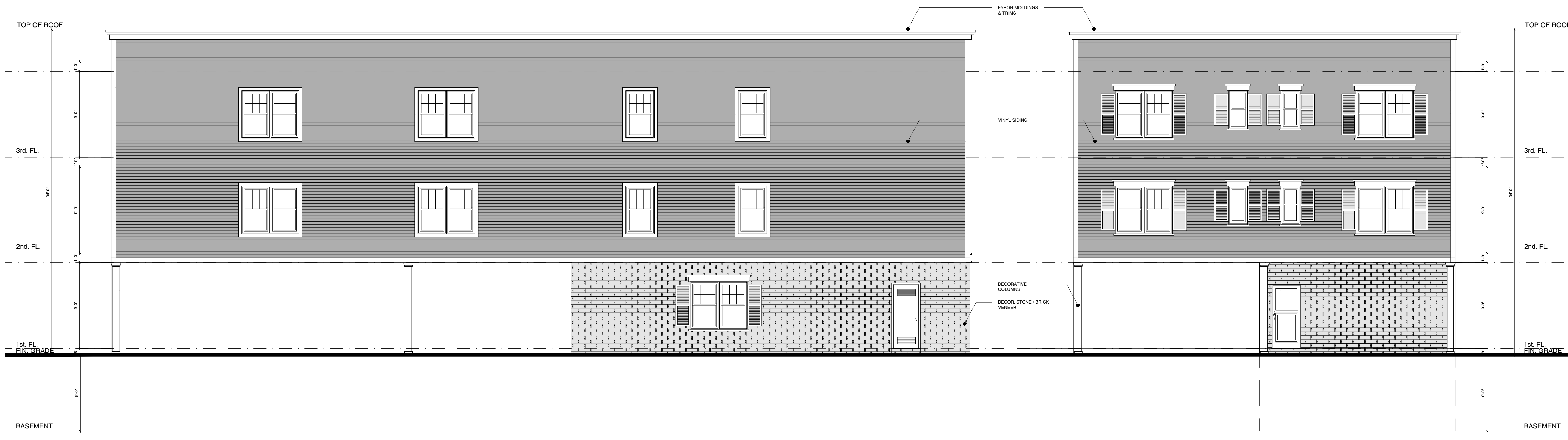
LEFT SIDE ELEVATION SCALE: \frac{3}{16}'' = 1'-0''
