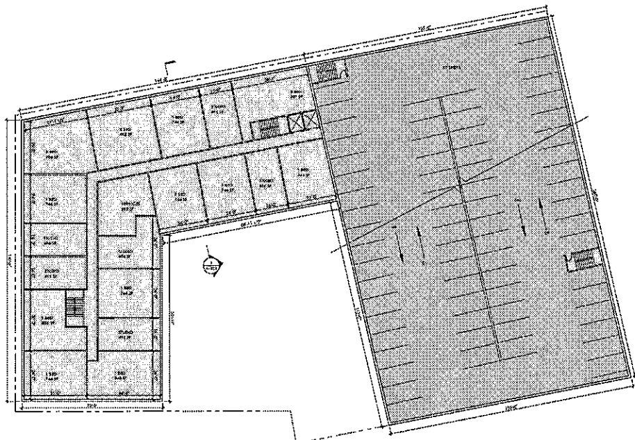
RESIDENTIAL FLOOR PLAN LEVEL 2 SCALE: 1/8" = 1'-0"
