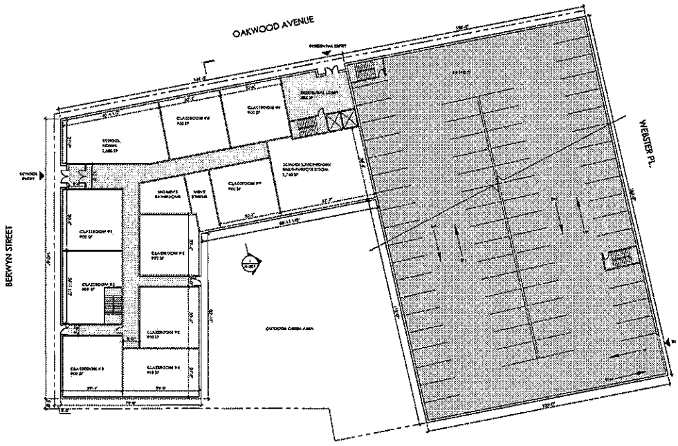
GROUND FLOOR PLAN Scale: 1/8" = 1'-0"
