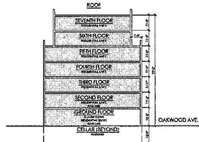
1 SECTION SCALE 1/8" = 1'-0"
