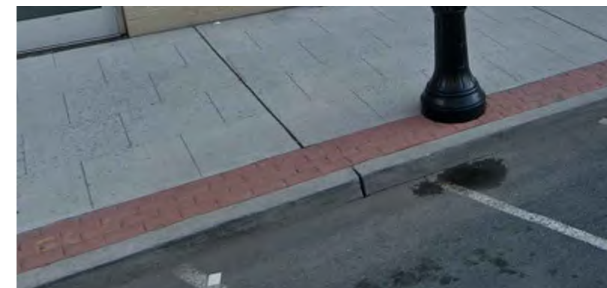
SCORED SIDEWALK WITH STAMPED BORDER
